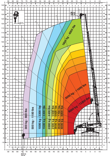
W 6 Argano 6 tonnellate
