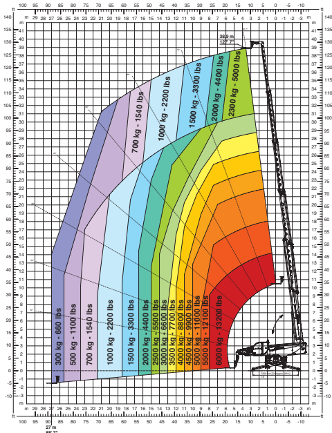
H 6 Gancio 6 tonnellate
