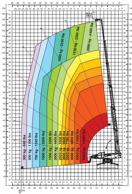
W 6 Argano 6 tonnellate
